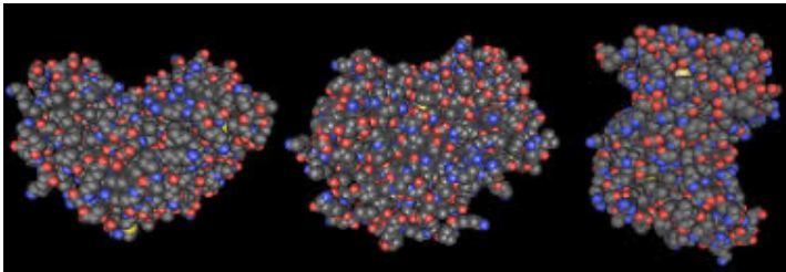
DNA Repairing Enzyme 'Experienced' Protein (quaternary structure)
