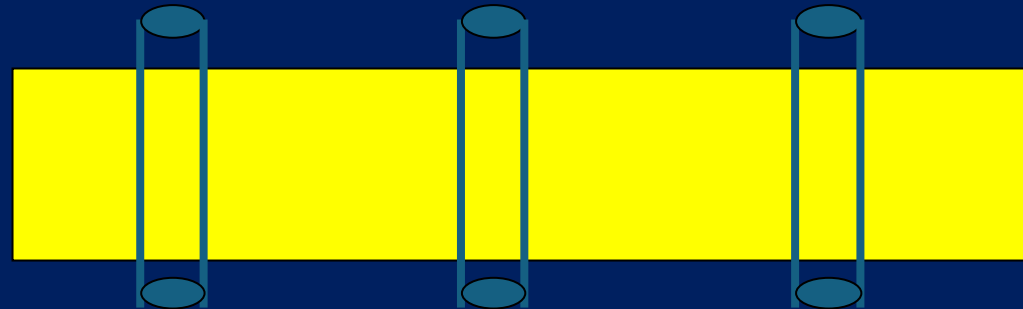
Quantum Mechanical Tunneling
